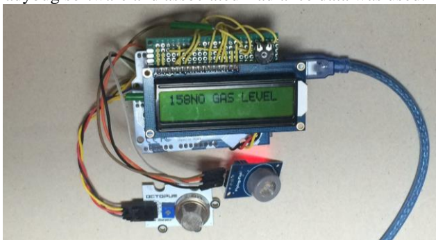
Fig. 4 Arduino microprocessor based sensor platform with gas sensors (Image by BettyLou Poston)
